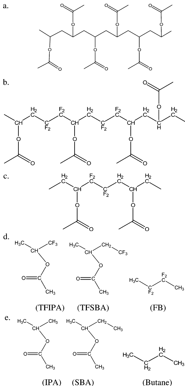
Figure 4. (a) PVAc; (b) a portion of poly(TFE-co-VAc) that lacks TFE block segments; (c) a representative segment of this copolymer; (d) the three small molecules used in molecular modeling that capture the features of the copolymer: trifluoroisopropyl acetate, trifluoro- sec -butyl acetate, and tetrafluorobutane; (e) the hydrocarbon analogues of the small fluororous molecules: isopropyl acetate, sec -butyl acetate, and n -butane.
