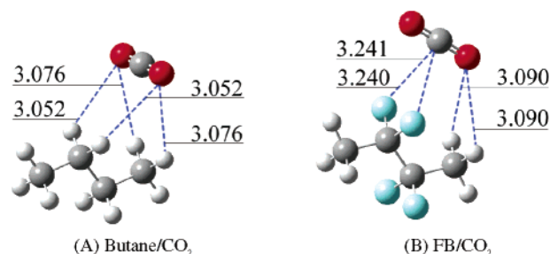
Figure 9. Optimized binding geometries for the n -butane/CO 2 (A) and FB/CO 2 (B) systems. Distances are in angstroms.
